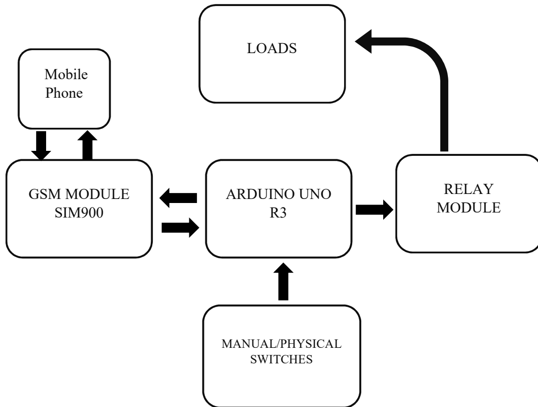
Figure 13: Block Diagram
