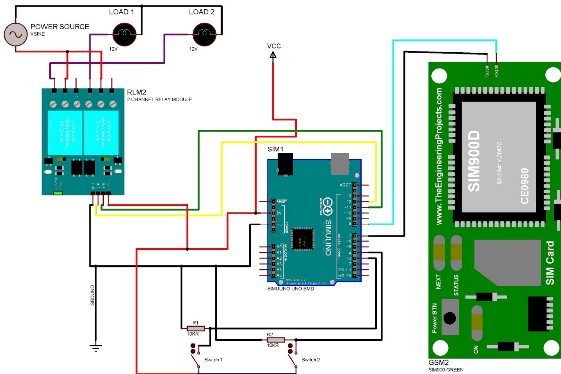
Figure 12: Circuit Breaker
